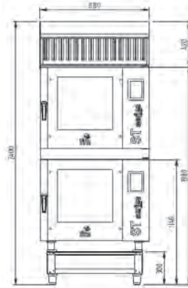
HOOD ST ST 606 ST 606 STAND ST 300 KIT SUPERPOSITION SERIES ST
